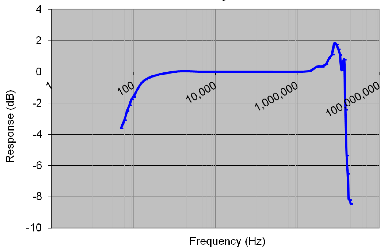
100A Rogowski Probe
